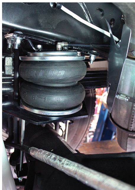
Passenger's (right) side inside frame view
