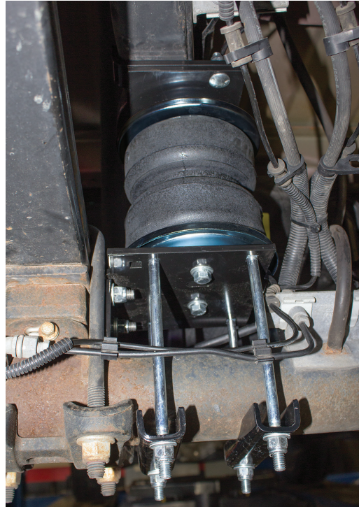
fig. 32 Left (driver's) side: rear view of installation.
