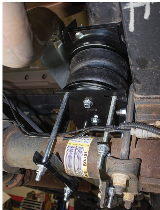
fig. 34 Right (passenger's) side: front view of installation.
